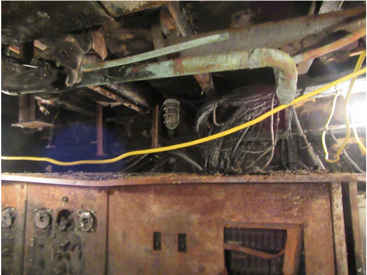
Generator Distribution Panel
