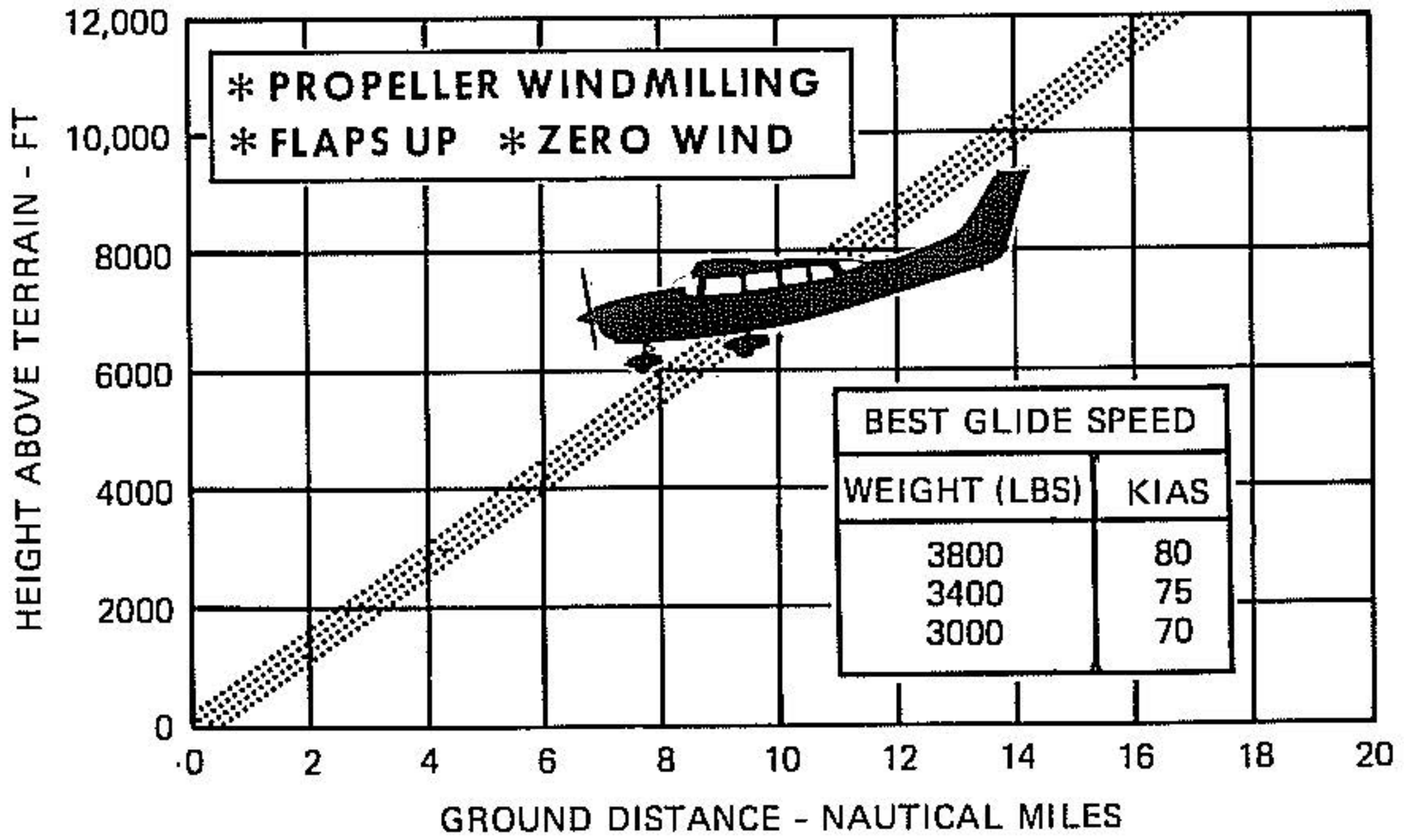
Figure 3-1. Maximum Glide
