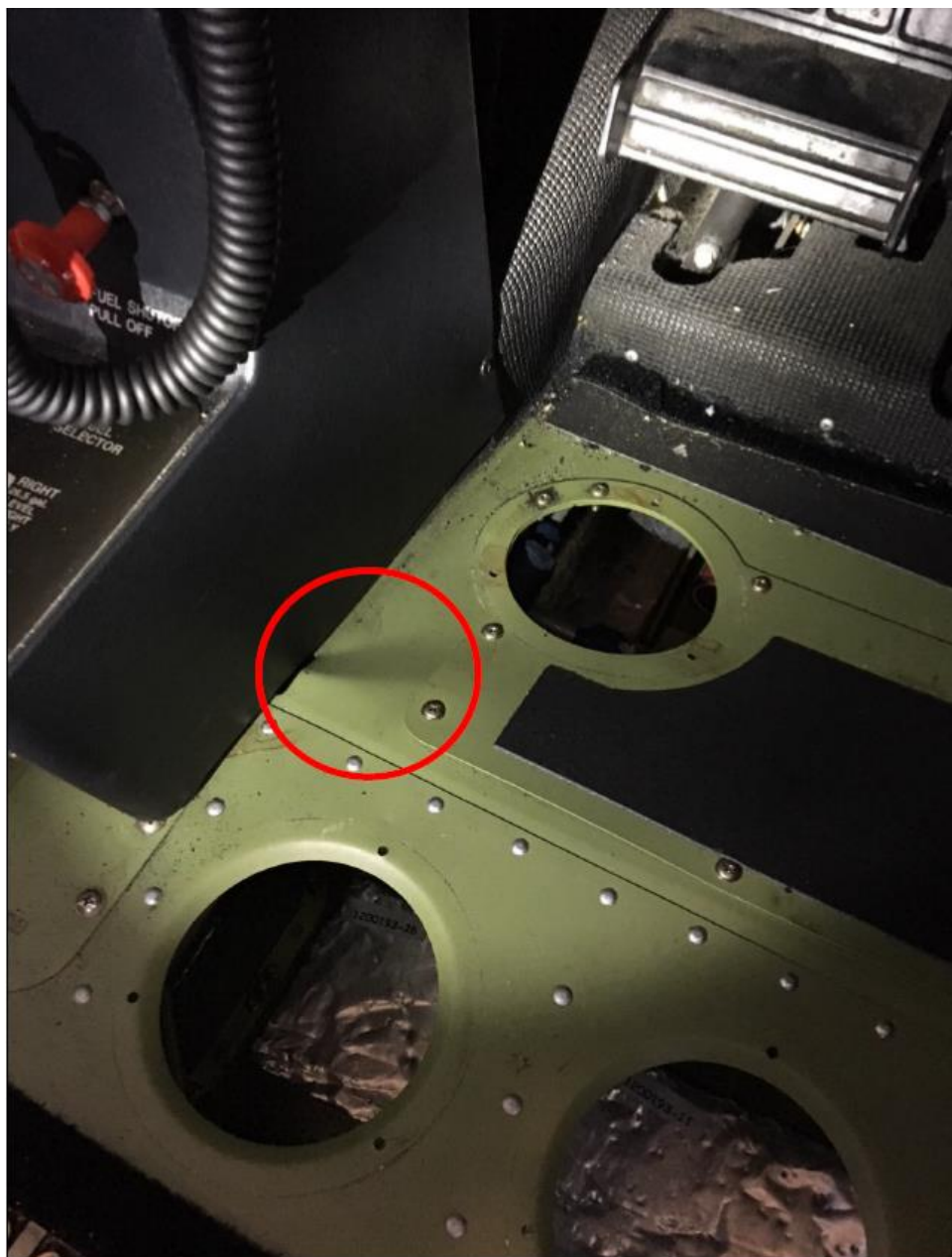
Photo 2 - View of right cabin floor panel (Photo courtesy of the FAA)
