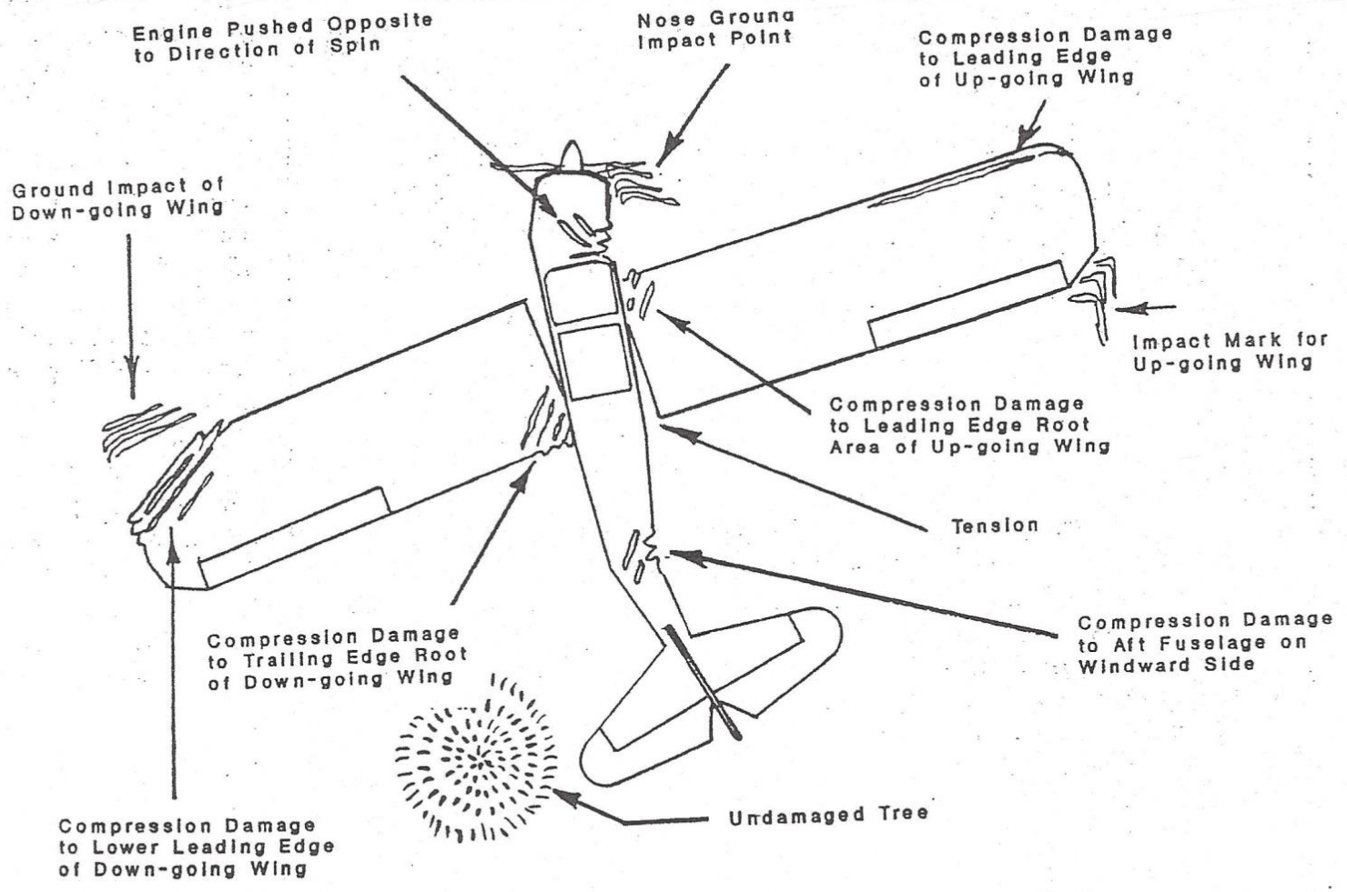
Figure 27-17. Wreckage Pattern of a Spinning Airplane
