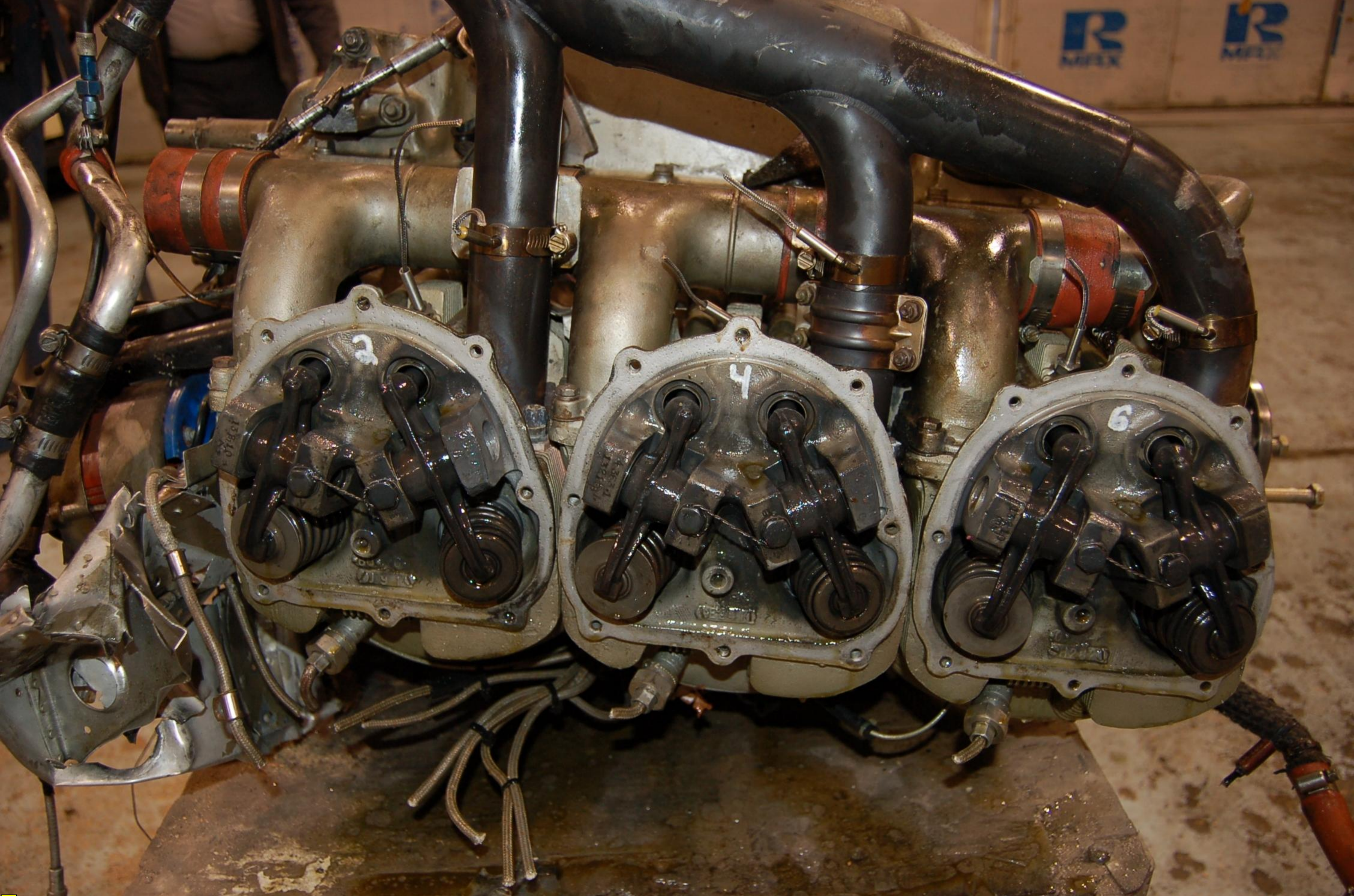
Photograph # 9 – View of 2-4-6 side of engine cylinder assemblies.
