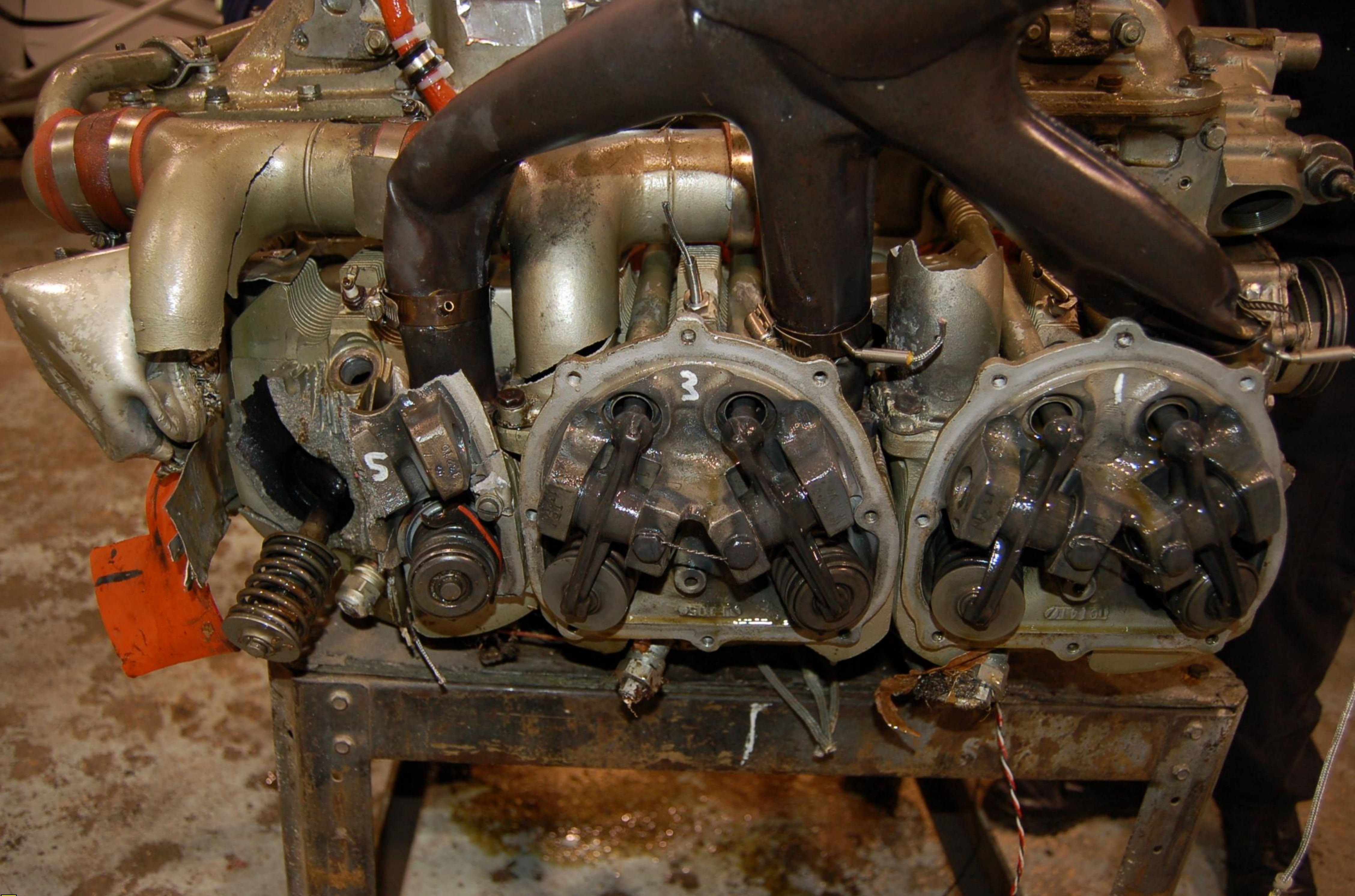
Photograph # 8 – View of 1-3-5 side of engine cylinder assemblies.
