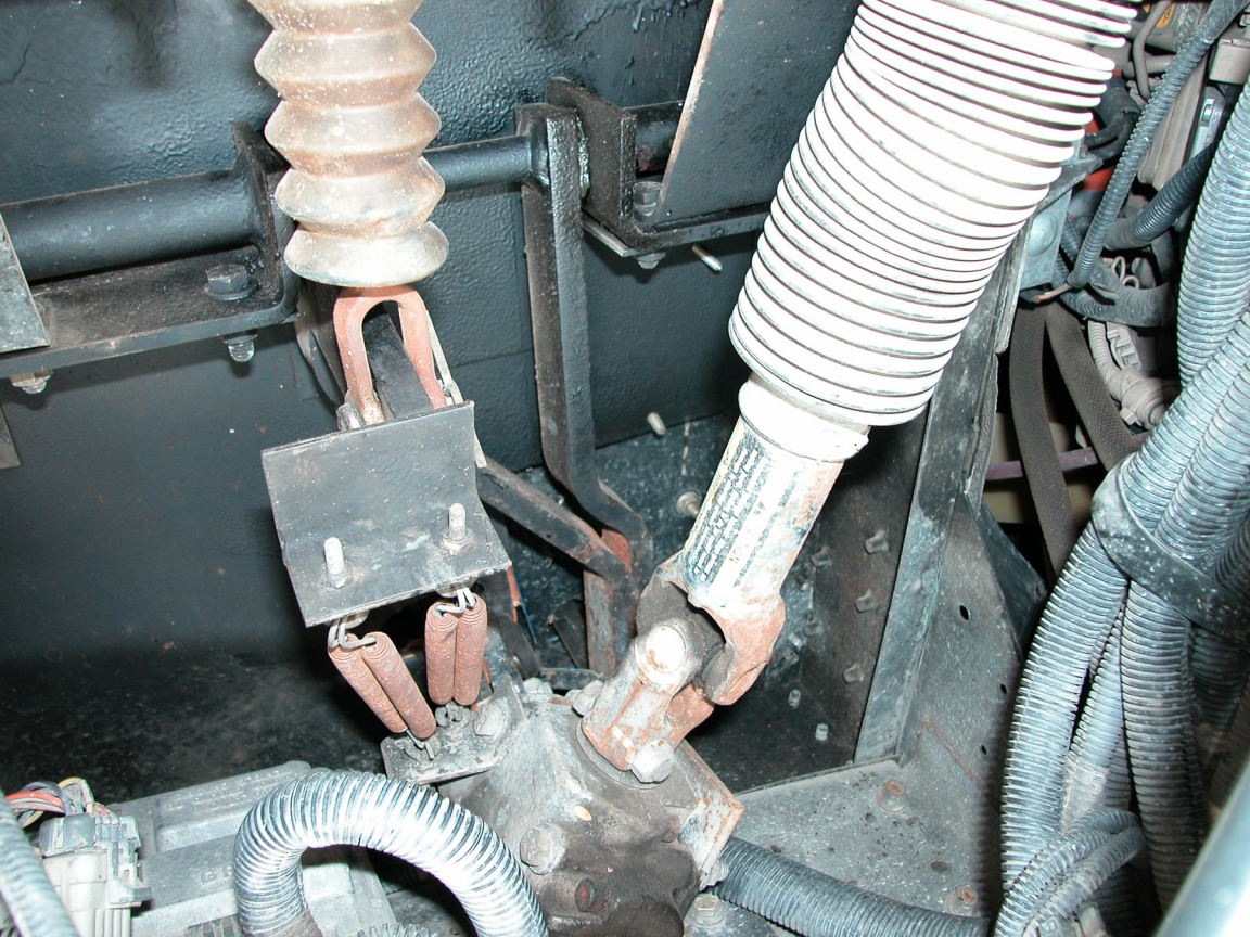
Vehicle Photo 15 – 2001 Blue Bird School Bus, Non-standard Spring Assembly
