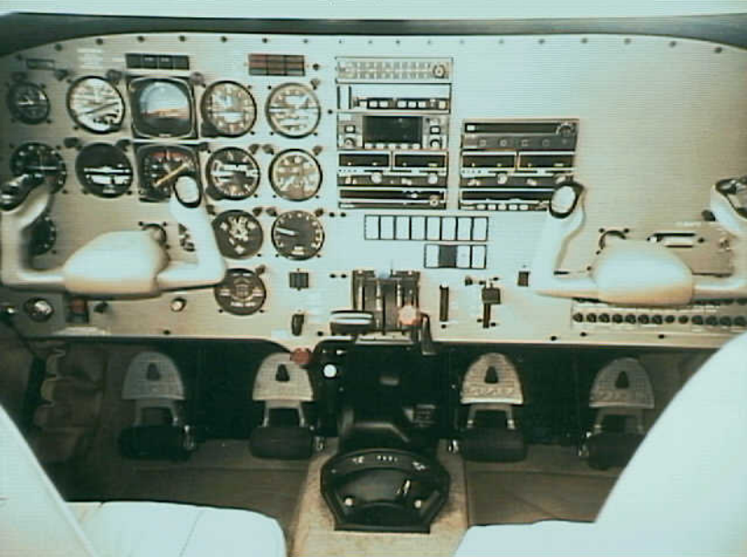
Photo 3. Photograph showing the interior cabin of the accident taken within three months of the accident. Second row of seats were aft-facing. (Photograph provided by previous owner of accident airplane)
