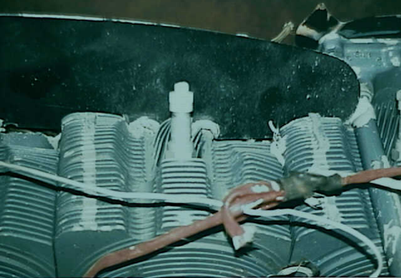
Airworthiness - Photo 28. Close-up view of the top of the no. 1 cylinder head section (view looking inboard) with propeller blade no. 1 resting next to it. Note consistent locations of blade damage with the cylinder damage. (NTSB-AA)
