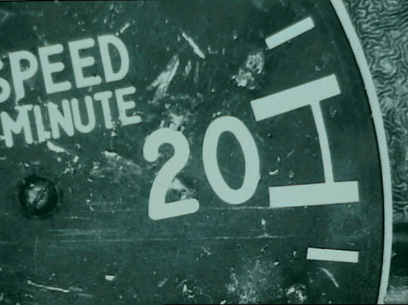
Airworthiness - Photo 21. Close-up view of the engine tachometer after removal from wreckage. Note that needle is captured at the 2,750 rpm indications, and the tachometer time reads 663.5 hours. (NTSB-T1)
