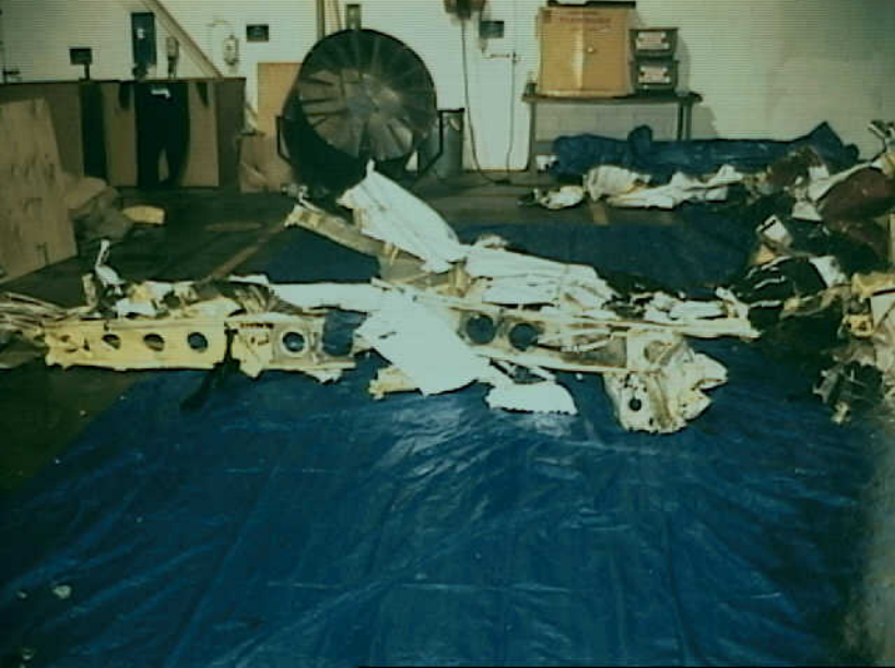
Airworthiness - Photo 4. Close-up view of the outboard portion of the right wing (view from forward looking aft). Note aftward accordion crush damage of the leading edge skin. (NTSB-C13)
