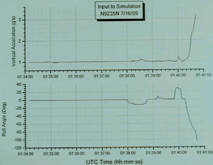
Aircraft Performance 13 - Attachment 3 - Chart 1 - Input to Simulation 7/16/99
