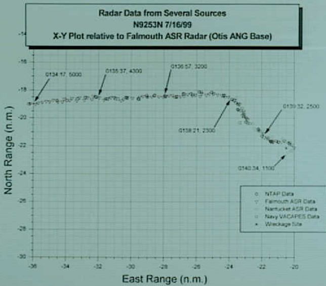
Aircraft Performance 13 - Attachment 1 - Chart 3 - Selected Final Radar Returns for N9253N
