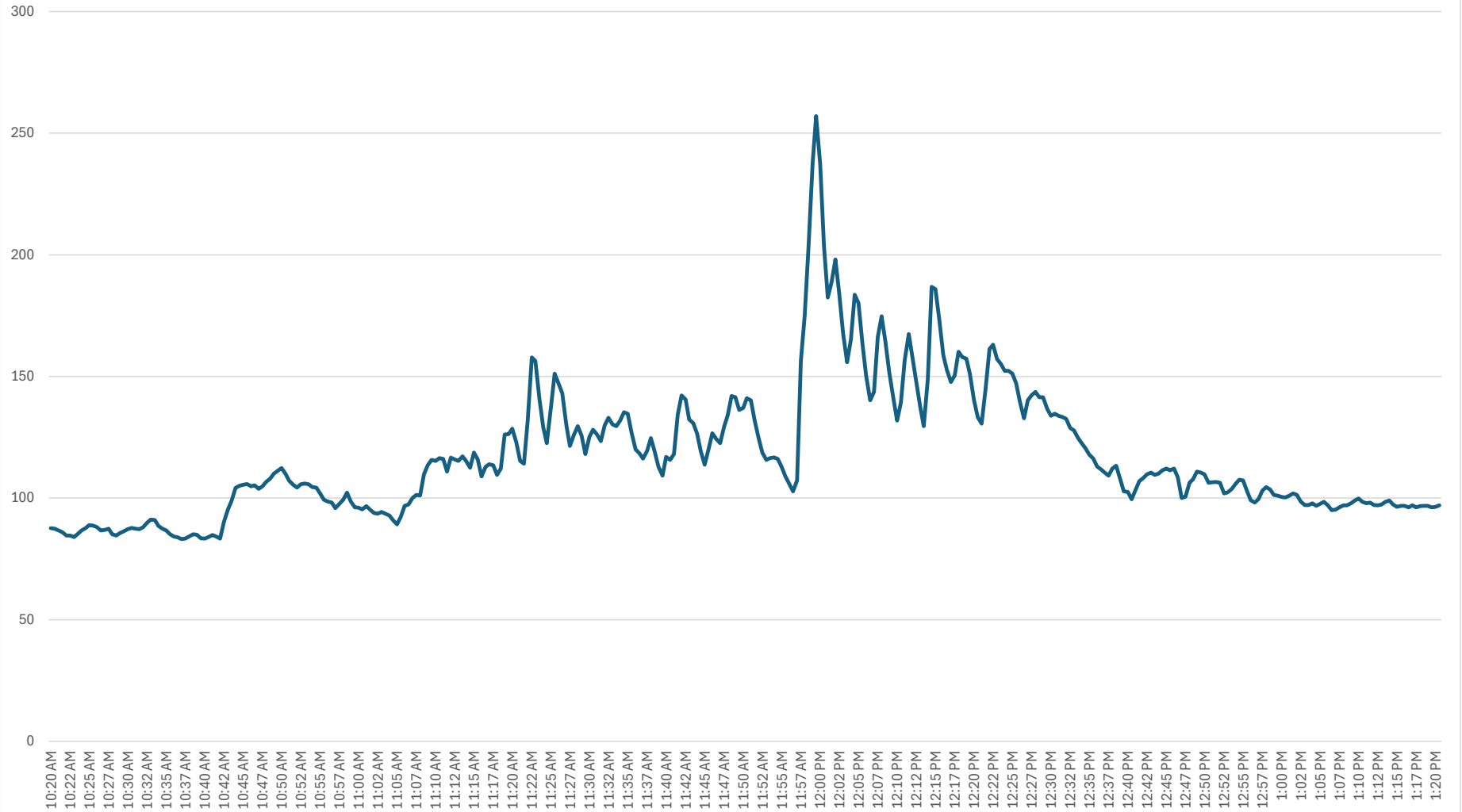
Test Train Trip Temperature Data Recorded Near Resistor Bank 6 (°F)
