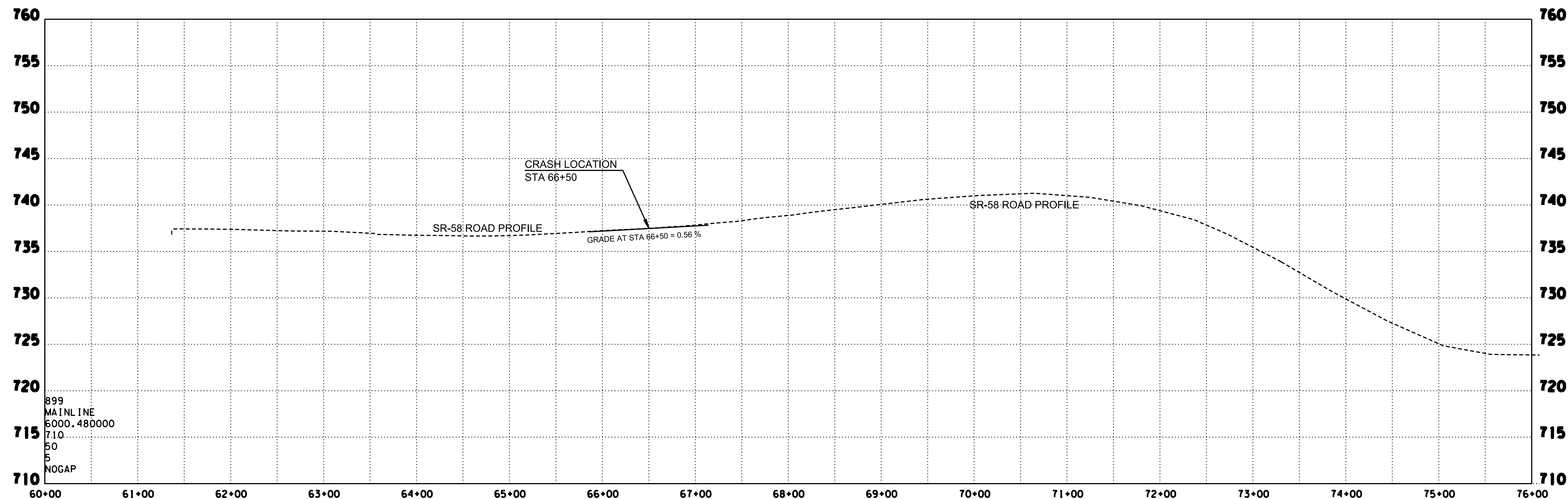
SR-58 CENTERLINE PROFILE V.E. X 10
