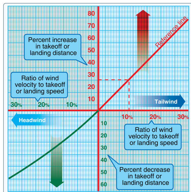
Figure 11-19. Effect of wind on takeoff and landing.
