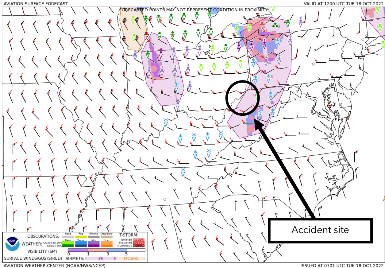
Figure 1. GFA Surface Forecast valid at 0800 EDT with forecast issued at 0301 EDT.
