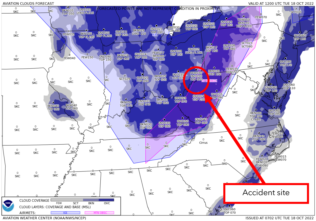
Figure 3. GFA Aviation Clouds Forecast valid at 0800 EDT with forecast issued at 0302 EDT.
