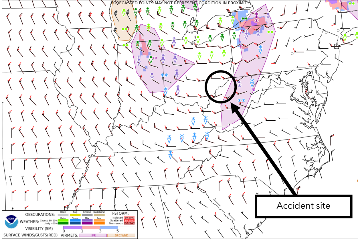
Figure 2. GFA Surface Forecast valid at 0800 EDT with forecast issued at 0601 EDT.
