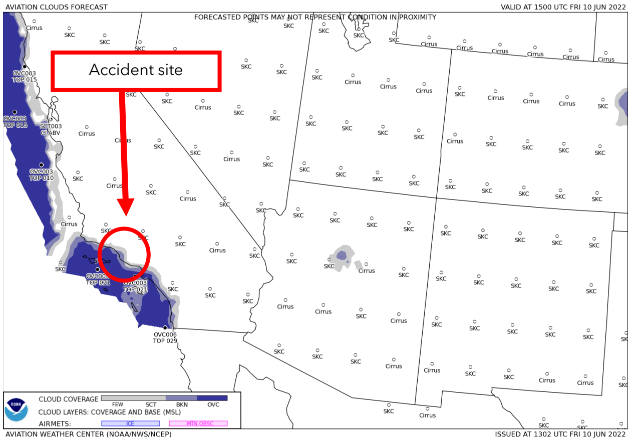
Figure 4. GFA Aviation Clouds Forecast valid at 0800 PDT with forecast issued at 0602 PDT.
