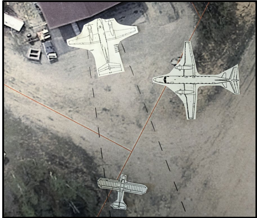
Figure 9 and 10: Representation Showing the Location the Airplane's Left Wing Contacted the Runway and after it was Spun
