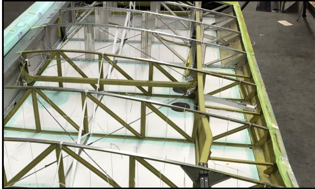
Figure 3: Damage to the Wing Spar
