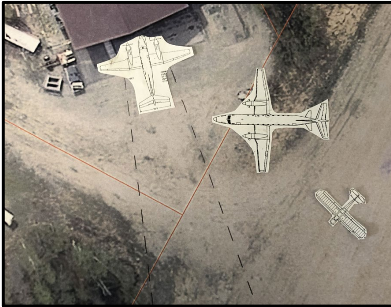
Figure 6 and 7: Representation Showing the Turn and Initial Encounter of the Wind Produced by the Turbo-Prop Airplane's Propellers
