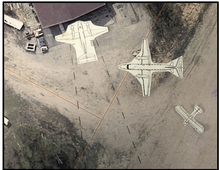
Figure 4 and 5: Representation Showing the Turn from the Runway to Taxiway ZZ
