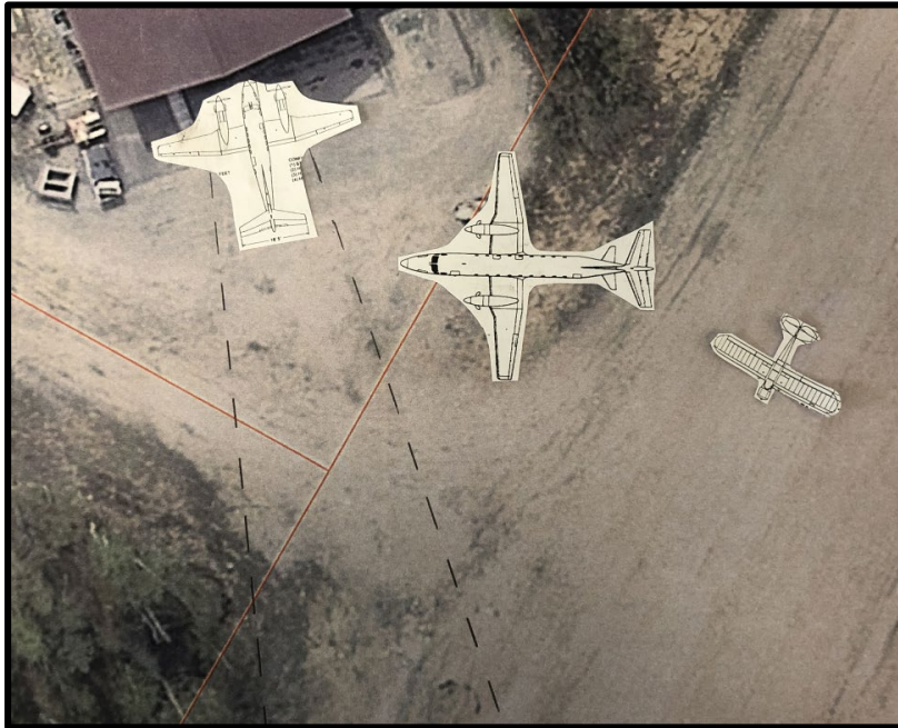
Figure 4 and 5: Representation Showing the Turn from the Runway to Taxiway ZZ
