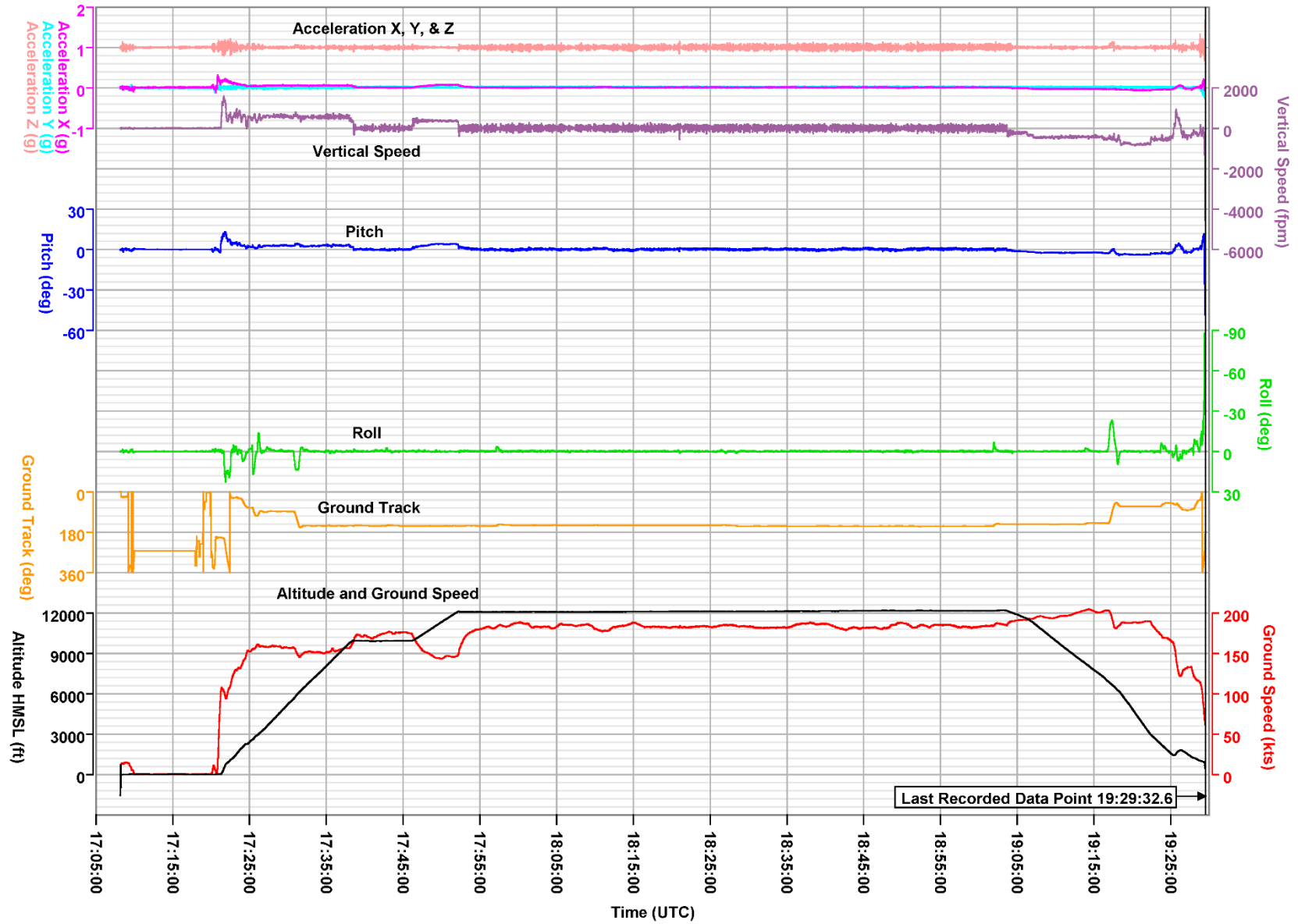
Basic parameters recorded on the Appareo Stratus for the entire accident flight
