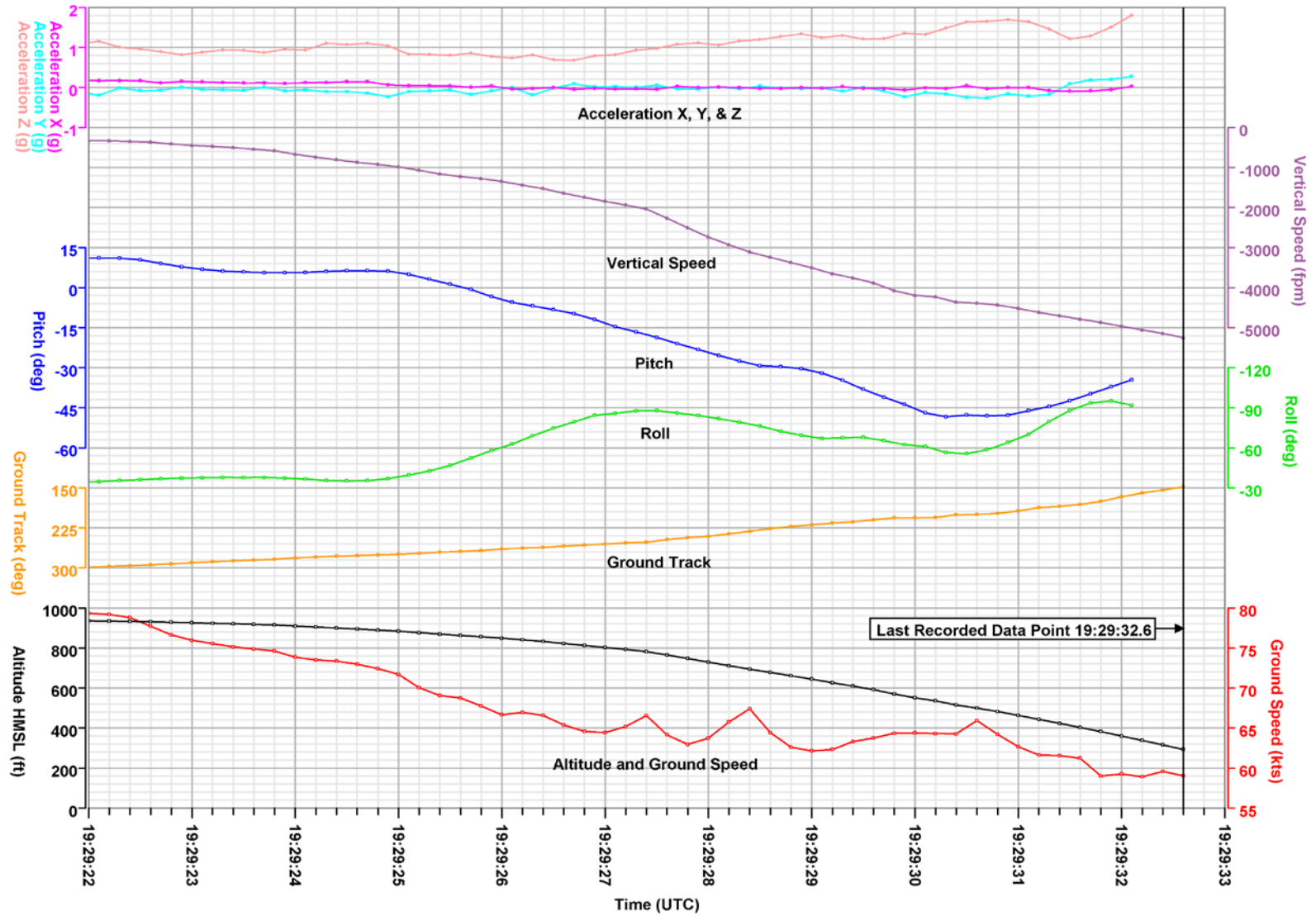
Basic parameters recorded on the Appareo Stratus at the end of the accident flight
