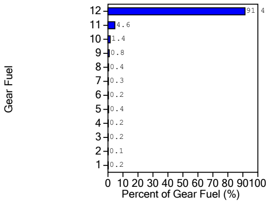
Forward Gear Fuel Histogram
