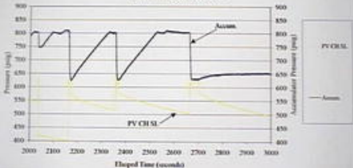
September 21, 2000 HP Exemplar Pilot Valve Runs #8 through 11: Plot E
