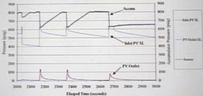
September 21, 2000 IEP Exemplar Pilot Valve Runs 88 through 11: Plot C
