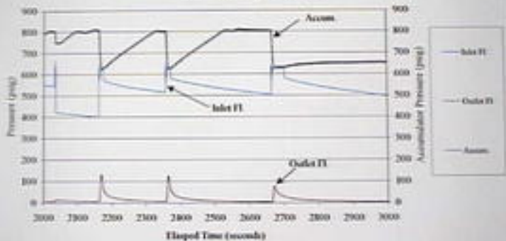
September 21, 2000 HP Exemplar Pilot Valve Runs #8 through 11: Plot B
