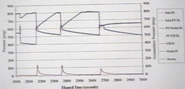
September 21, 2000 HP Exemplar Pilot Valve Runs #8 through 11: Plot A
