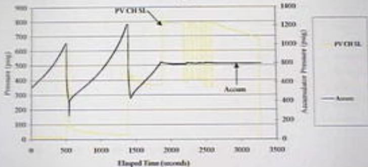
September 21, 2000 LP Exemplar Pilot Valve with Adjusted Set-Point Runs #7 through 14: Plot E
