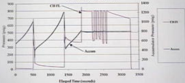
September 21, 2000 LP Exemplar Fillet Valve with Adjusted Set-Point Runs #7 through 14: Plot D
