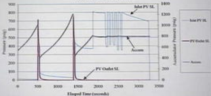
September 21, 2000 LP Exemplar Pilot Valve with Adjusted Set-Point Runs #7 through 14: Plot C
