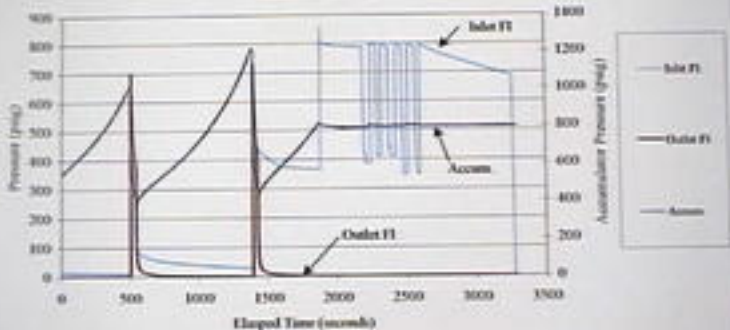
September 21, 2000 LP Exemplar Pilot Valve with Adjusted Set-Point Runs #7 through 14: Plot B
