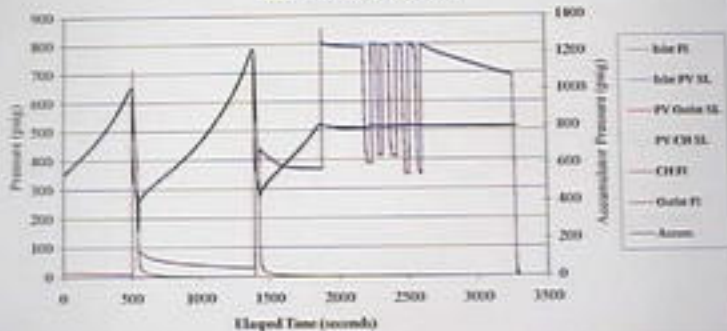
September 21, 2000 LP Exemplar Pilot Valve with Adjusted Set-Point Runs #7 through 14: Plot A
