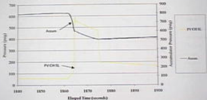
September 21, 2000 LP Exemplar Pilot Valve with Adjusted Set-Point Run #6: Plot E
