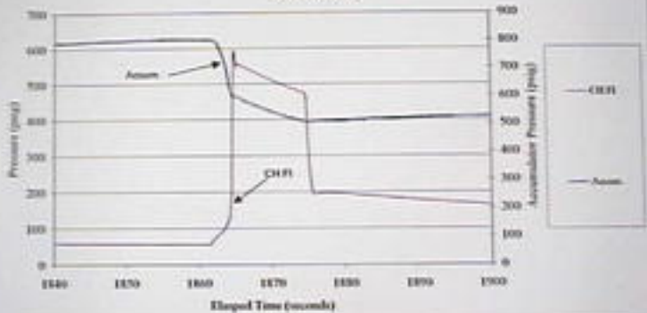
September 21, 2000 LP Exemplar Pilot Valve with Adjusted Set-Point Run #6: Plot D
