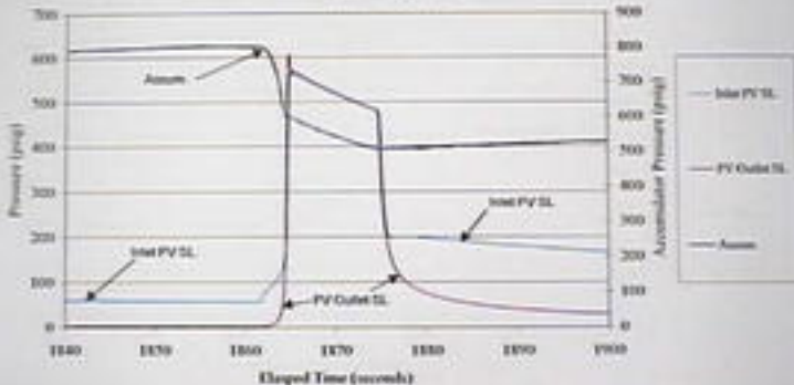
September 21, 2000 LP Exemplar Pilot Valve with Adjusted Set-Point Run #6; Plot C
