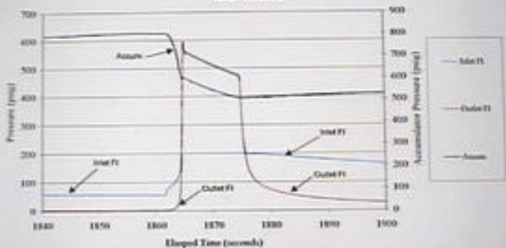
September 21, 2000 LP Exemplar Pilot Valve with Adjusted Set-Point Run #6: Plot B
