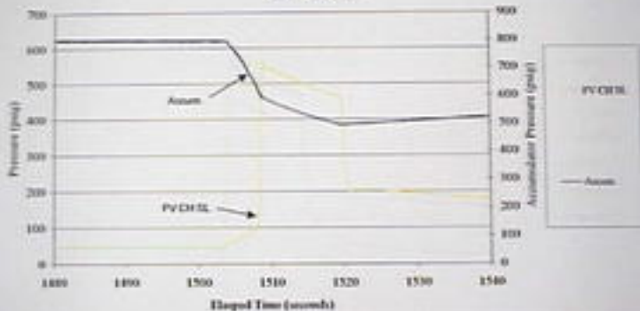
September 21, 2000 LP Exemplar Pilot Valve with Adjusted Set-Point Run #5: Plot E
