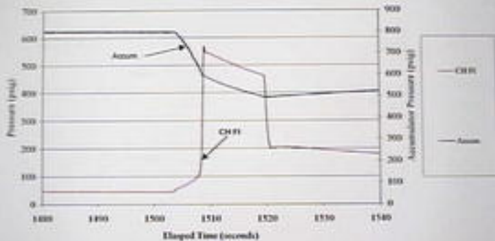
September 21, 2000 LP Exemplar Pilot Valve with Adjusted Set-Point Run #5: Plot D
