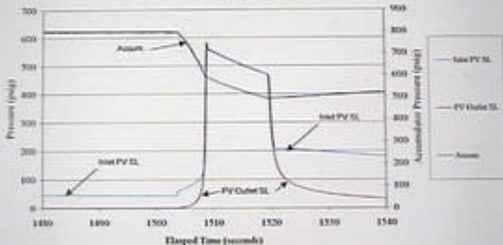
September 21, 2000 LP Exemplar Pilot Valve with Adjusted Set-Point Run #5: Plot C
