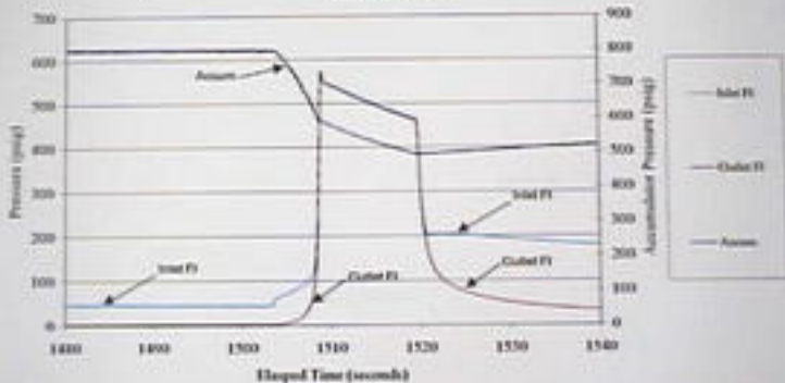
September 21, 2000 LP Exemplar Pilot Valve with Adjusted Set-Point Run #5: Plot B
