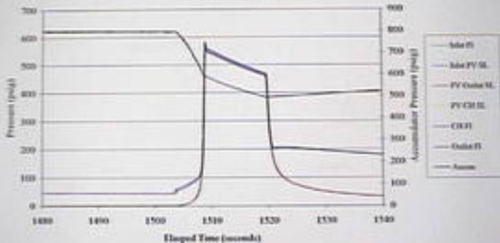
September 21, 2000 LP Exemplar Pilot Valve with Adjusted Set-Point Run #5: Plot A
