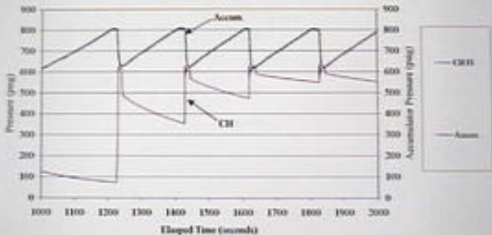
September 21, 2000 HP Exemplar Pilot Valve Runs #4 through 7: Plot D
