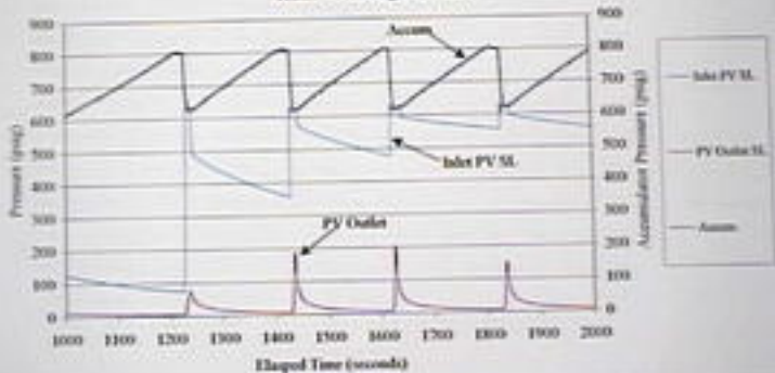
September 21, 2000 IIP Exemplar Pilot Valve Runs #4 through 7: Plot C
