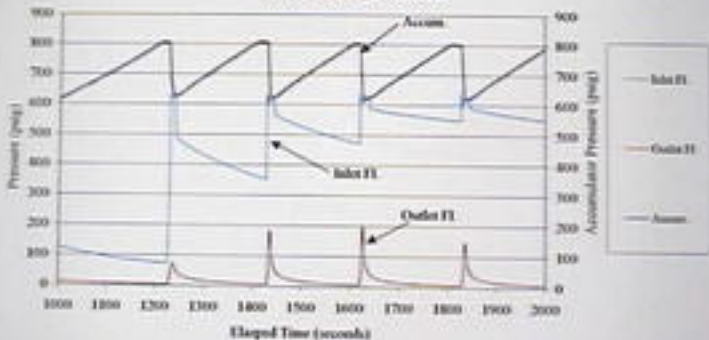
September 21, 2000 HP Exemplar Pilot Valve Runs #4 through 7: Plot B
