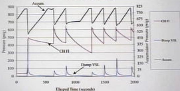
September 20, 2000 HP Exemplar Pilot Valve Runs #3 through 9: Plot D
