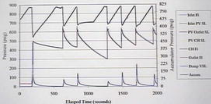
September 20, 2000 HP Exemplar Pilot Valve Runs #3 through 9: Plot A
