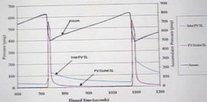
September 21, 2000 LP Exemplar Pilot Valve with Adjusted Set-Point Runs #3 through 4: Plot C
