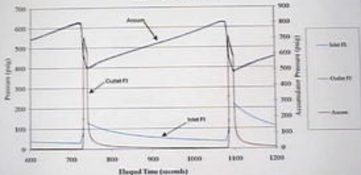
September 21, 2000 LP Exemplar Pilot Valve with Adjusted Set-Point Runs #3 through 4: Plot B
