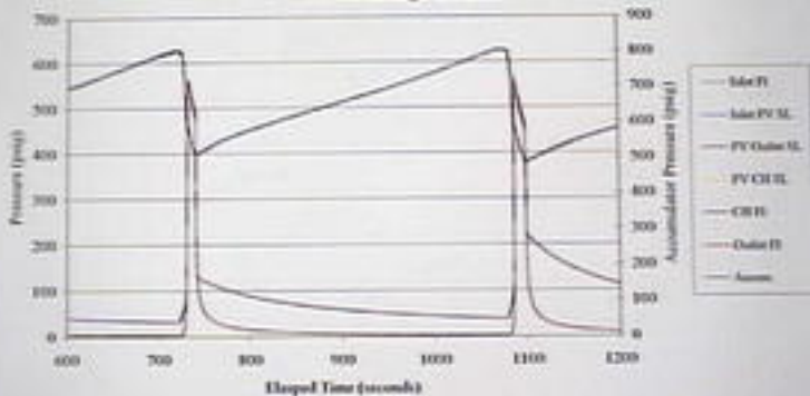
September 21, 2000 LP Exemplar Pilot Valve with Adjusted Set-Point Runs #3 through 4: Plot A
