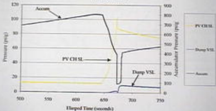
September 20, 2000 HIP Exemplar Pilot Valve Run #2: Plot E
