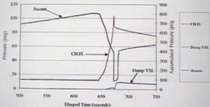
September 20, 2000 HP Exemplar Pilot Valve Run #2: Plot D
