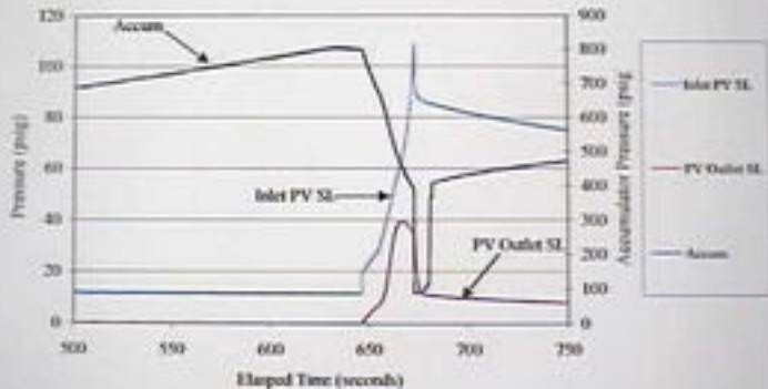
September 20, 2000 HP Exemplar Pilot Valve Run #2: Plot C
